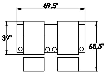
8137-11P 8137-04S 8137-12P (65.5*69.5*39)
