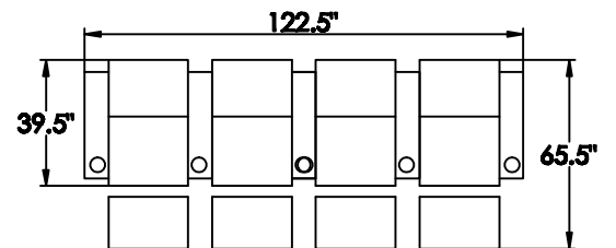
8137-11P 8137-11P 8137-11P 8137-08T/P (39.5*65.5*122.5)
